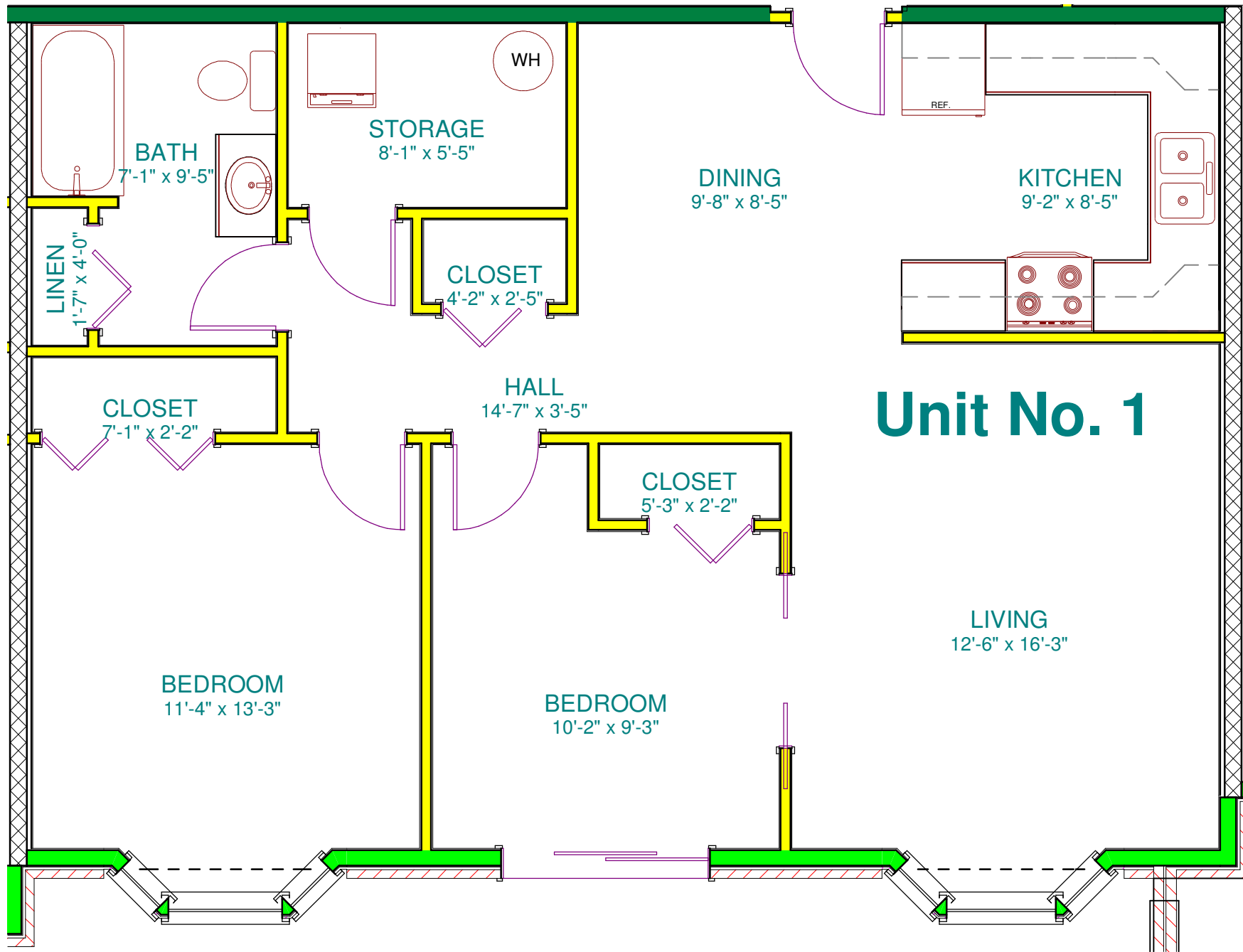
LLOYD HOUSE Scale: 1/4" = 1'-0"
